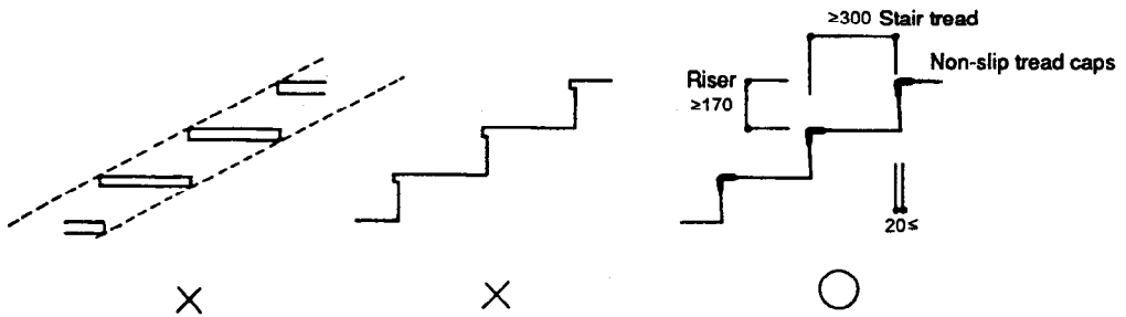
Stair dimensions
