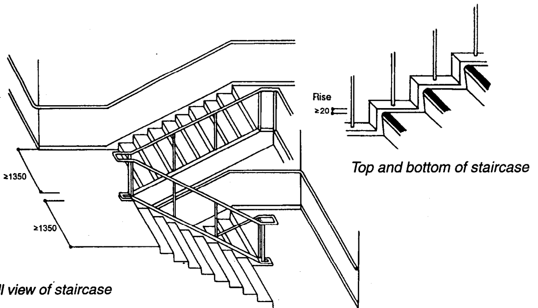
Stair dimensions
